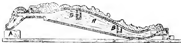
No. 132.—SECTION OF CAST OF BALCONY FRONT.
